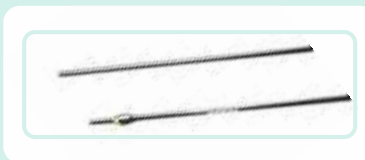
Product code HHW-06 Guide Wire with Ball for Interlocking Nails (Available in Different Length and Diameter)
